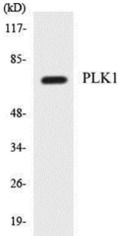
Figure 4. Western blot analysis of extracts from LOVO cells, treated with PMA 125ng/ml 30', using the Anti-PLK1 Antibody.
