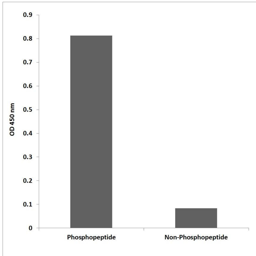
Figure 3. Enzyme-Linked Immunosorbent Assay (ELISA) for immunogen phosphor-peptide (left) and non-phospho peptide (right), using Anti-PLK1 (Phospho-Ser137) Antibody.
