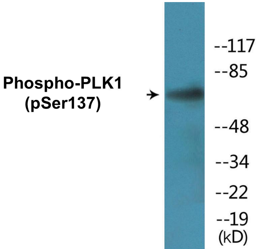
Figure 2. Western blot analysis of extracts from Jurkat cells treated with PMA, using the Anti-PLK1 (Phospho-Ser137) Antibody.
