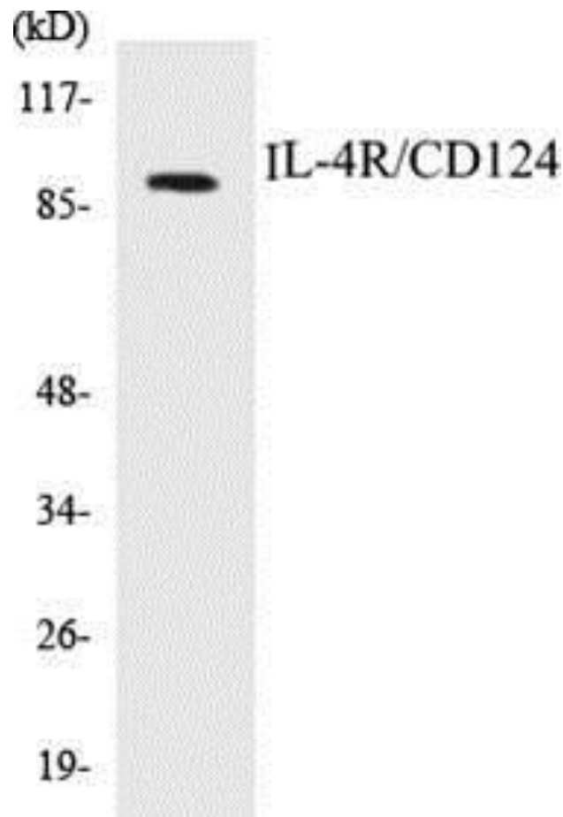
Figure 4. Western blot analysis of extracts from 293 cells, using the Anti-IL-4R/CD124 Antibody.
