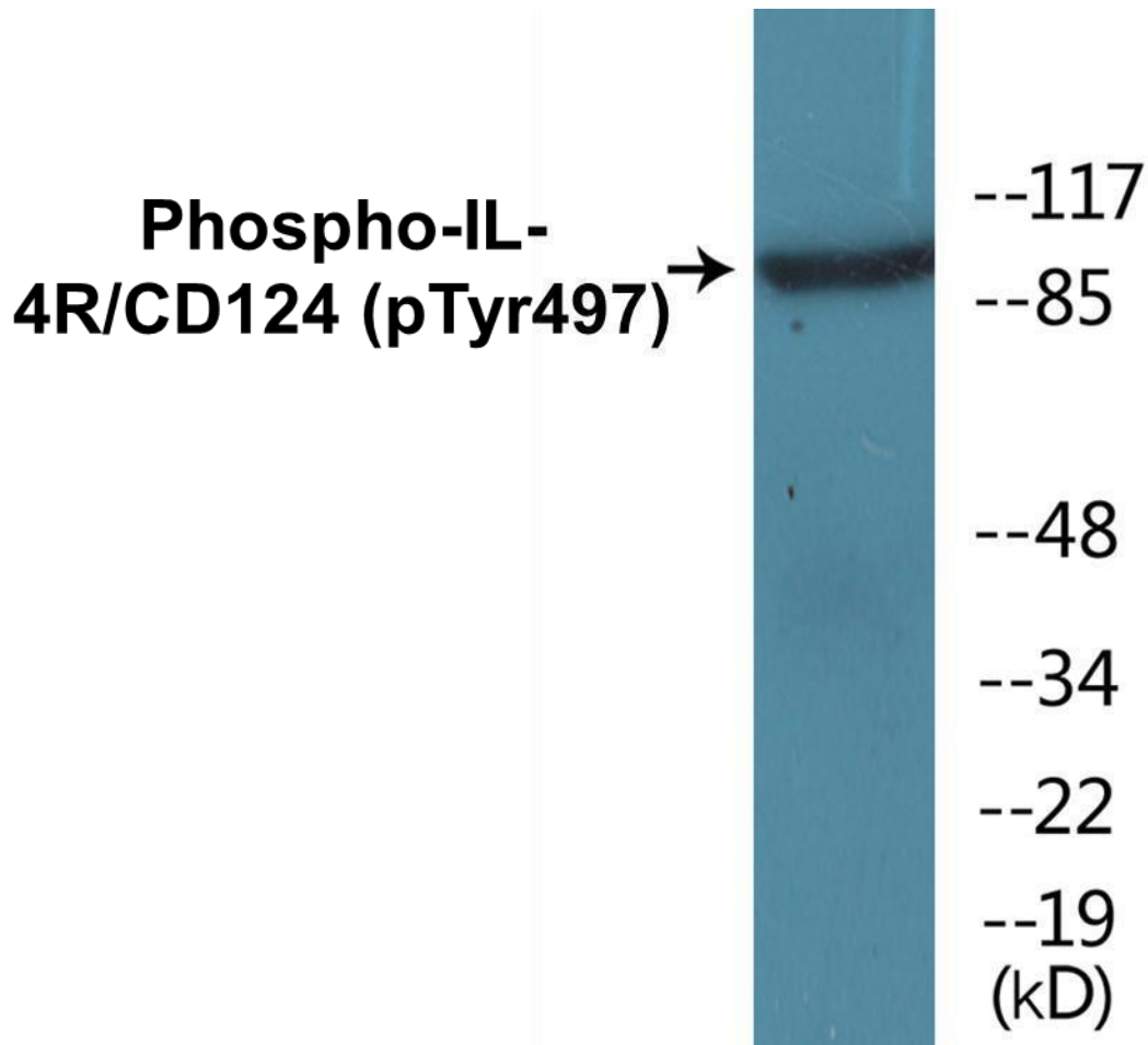
Figure 2. Western blot analysis of extracts from 293 cells, using the Anti-IL-4R/CD124 (Phospho-Tyr497) Antibody.
