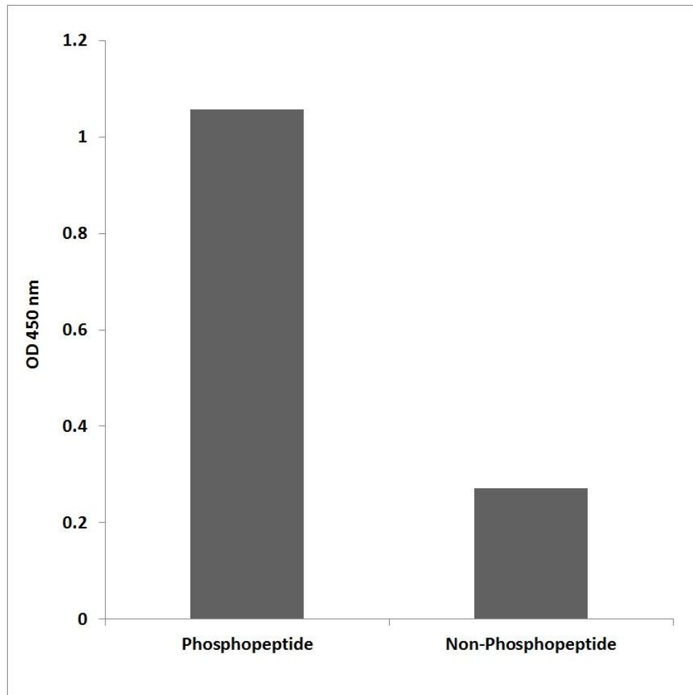
Figure 3. Enzyme-Linked Immunosorbent Assay (ELISA) for immunogen phosphor-peptide (left) and non-phospho peptide (right), using Anti-IL-4R/CD124 (Phospho-Tyr497) Antibody.
