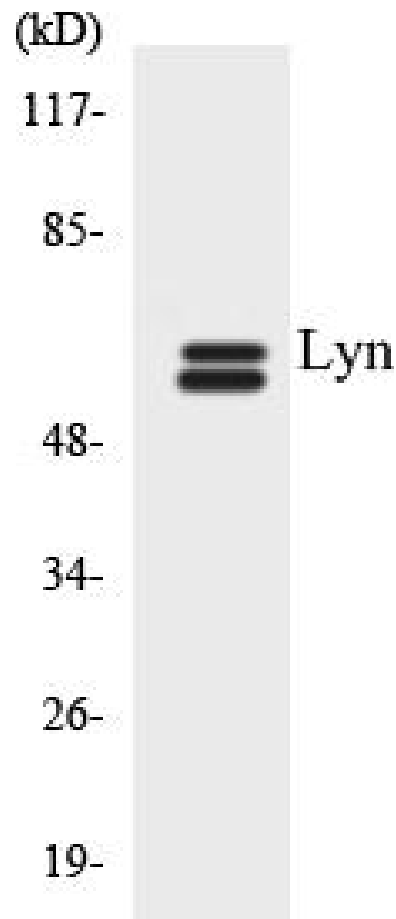
Figure 2. Western blot analysis of extracts from COLO cells, treated with H 2 O 2 100uM 30', using Lyn (Ab-507) Antibody.
