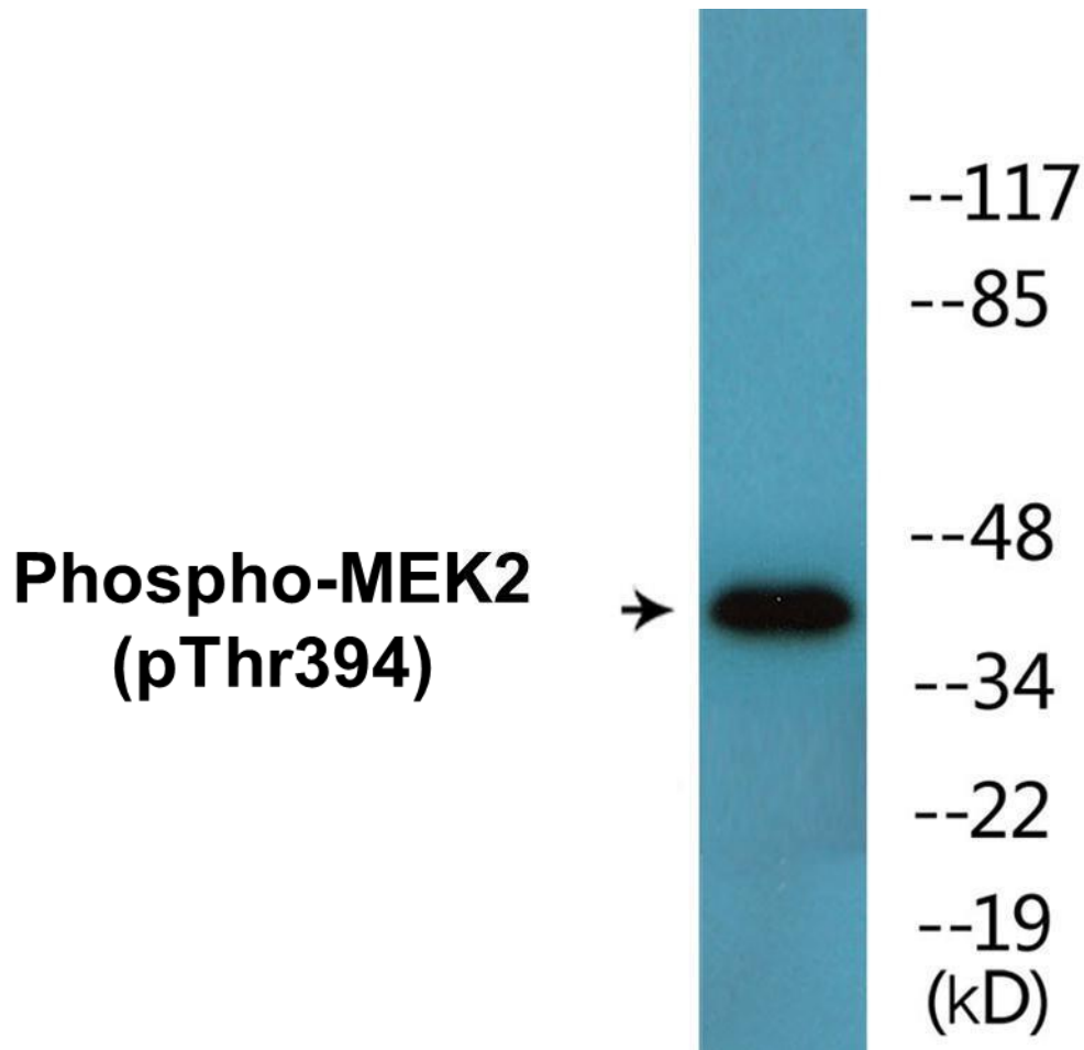
Figure 2. Western blot analysis of extracts from ovary cancer, using the Anti-MEK2 (Phospho-Thr394) Antibody.
