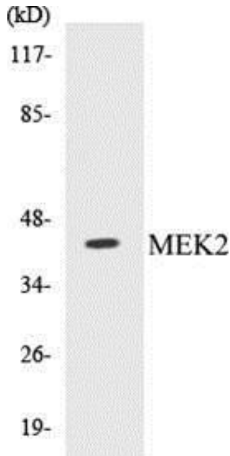
Figure 4. Western blot analysis of extracts from ovary cancer cells, using the Anti-MEK2 Antibody.
