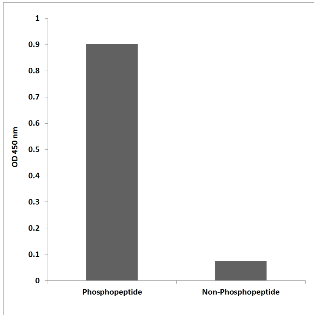
Figure 3. Enzyme-Linked Immunosorbent Assay (ELISA) for immunogen phosphor-peptide (left) and non-phospho peptide (right), using Anti-MEK2 (Phospho-Thr394) Antibody.
