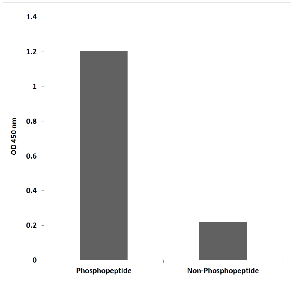
Figure 3. Enzyme-Linked Immunosorbent Assay (ELISA) for immunogen phosphor-peptide (left) and non-phospho peptide (right), using Anti-MEF2A (Phospho-Thr319) Antibody.
