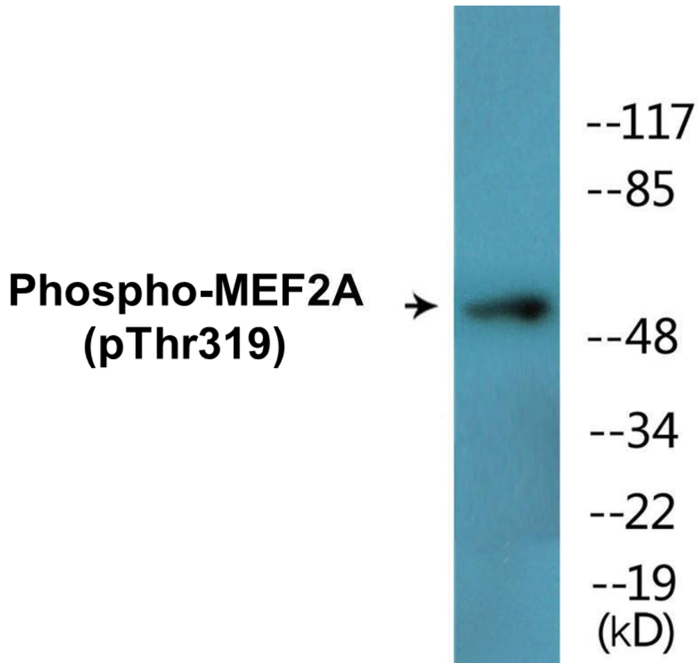
Figure 2. Western blot analysis of extracts from K562 cells treated with UV 15', using the Anti-MEF2A (Phospho-Thr319) Antibody.
