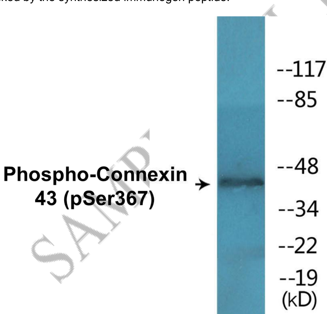
Figure 2. Western blot analysis of extracts from K562 cells treated with PMA 200ng/ml 10', using the Anti-Connexin 43 (Phospho-Ser367) Antibody.
