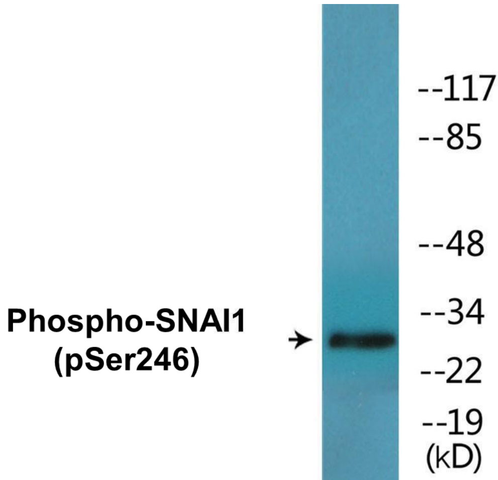
Figure 2. Western blot analysis of extracts from HT29 cells, using the Anti-SNAI1 (Phospho-Ser246) Antibody.
