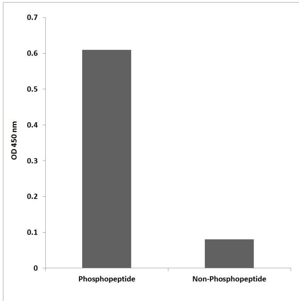
Figure 3. Enzyme-Linked Immunosorbent Assay (ELISA) for immunogen phosphor-peptide (left) and non-phospho peptide (right), using Anti-SNAI1 (Phospho-Ser246) Antibody.
