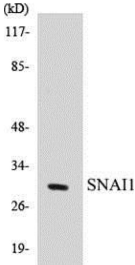
Figure 4. Western blot analysis of extracts from HT29 cells, using the Anti-SNAI1 Antibody.
