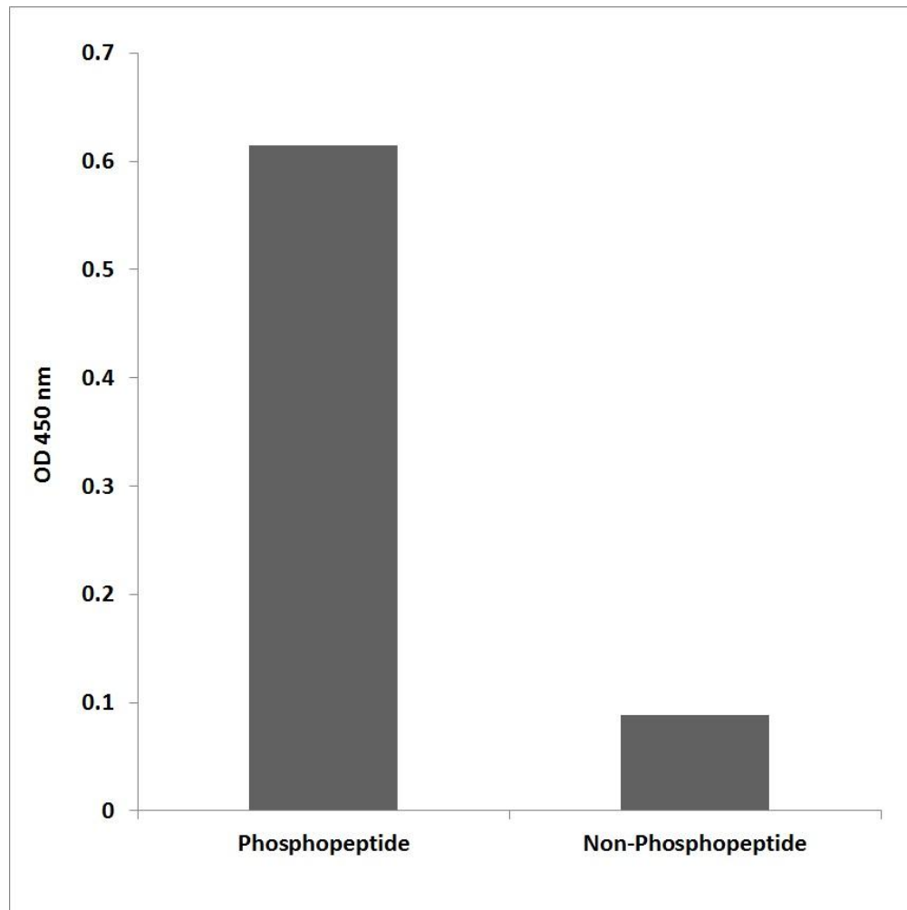
Figure 3. Enzyme-Linked Immunosorbent Assay (ELISA) for immunogen phosphor-peptide (left) and non-phospho peptide (right), using Anti-p95-NBS1 (Phospho-Ser278) Antibody.
