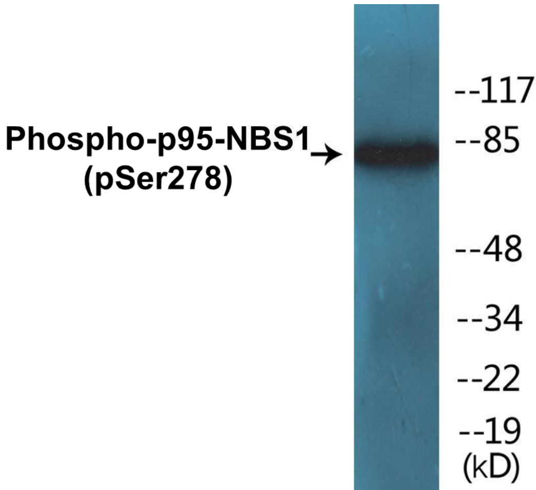
Figure 2. Western blot analysis of extracts from HuvEc cells treated with Forskolin 40nM 30', using the Anti-p95-NBS1 (Phospho-Ser278) Antibody.
