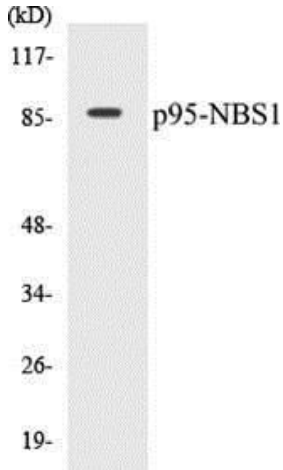
Figure 4. Western blot analysis of extracts from Jurkat cells, using the Anti-p95-NBS1 Antibody.
