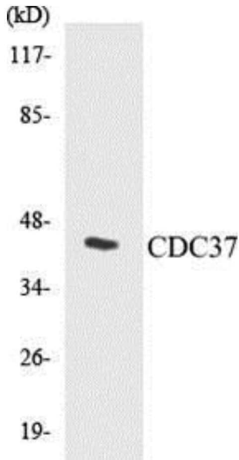
Figure 4. Western blot analysis of extracts from MCF-7/COS7 cells, using the Anti-CDC37 Antibody.
