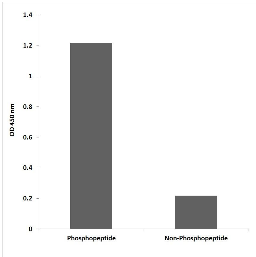
Figure 3. Enzyme-Linked Immunosorbent Assay (ELISA) for immunogen phosphor-peptide (left) and non-phospho peptide (right), using Anti-CDC37 (Phospho-Ser13) Antibody.
