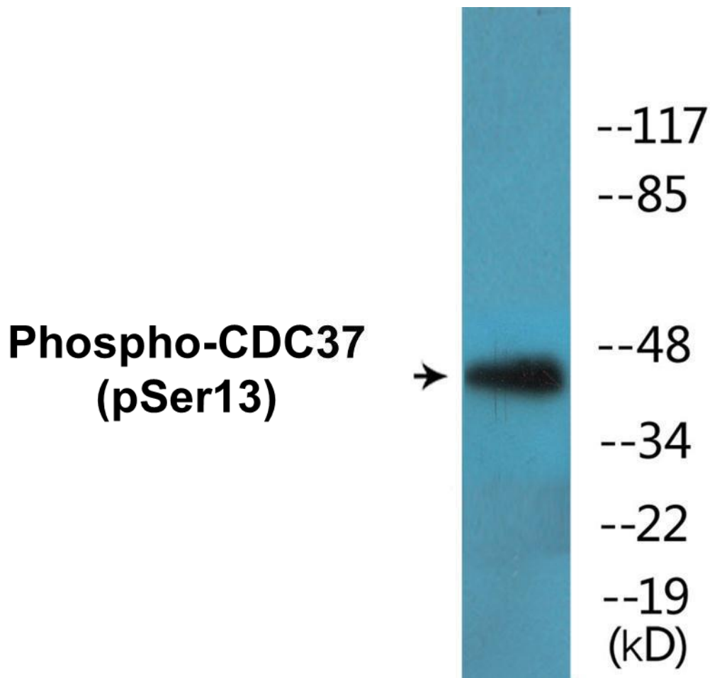
Figure 2. Western blot analysis of extracts from HuvEc cells, using the Anti-CDC37 (Phospho-Ser13) Antibody.
