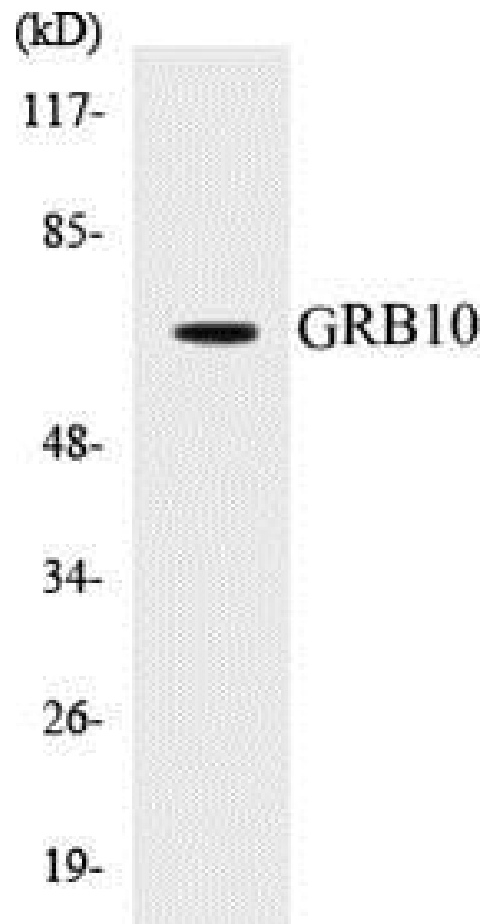
Figure 4. Western blot analysis of extracts from NIH-3T3 cells, treated with Insulin 0.01U/ml 15', using the Anti-GRB10 Antibody.
