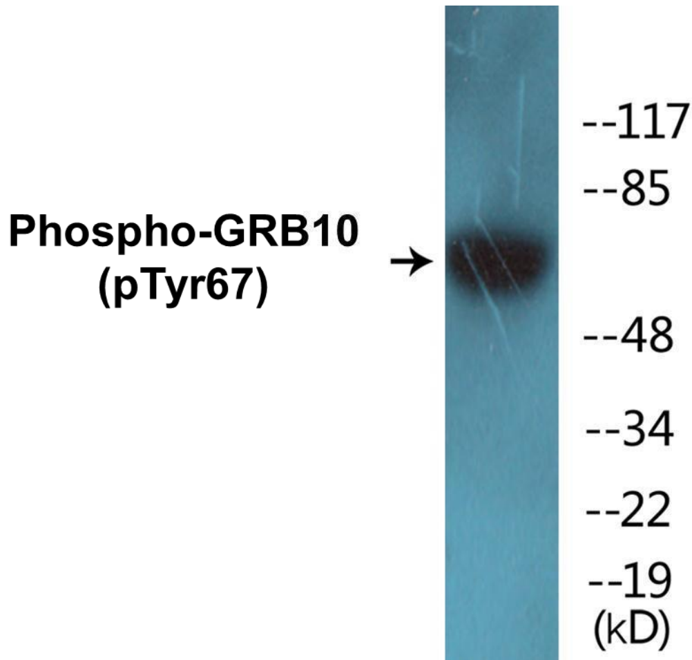
Figure 2. Western blot analysis of extracts from COS7 cells, using the Anti-GRB10 (Phospho-Tyr67) Antibody.
