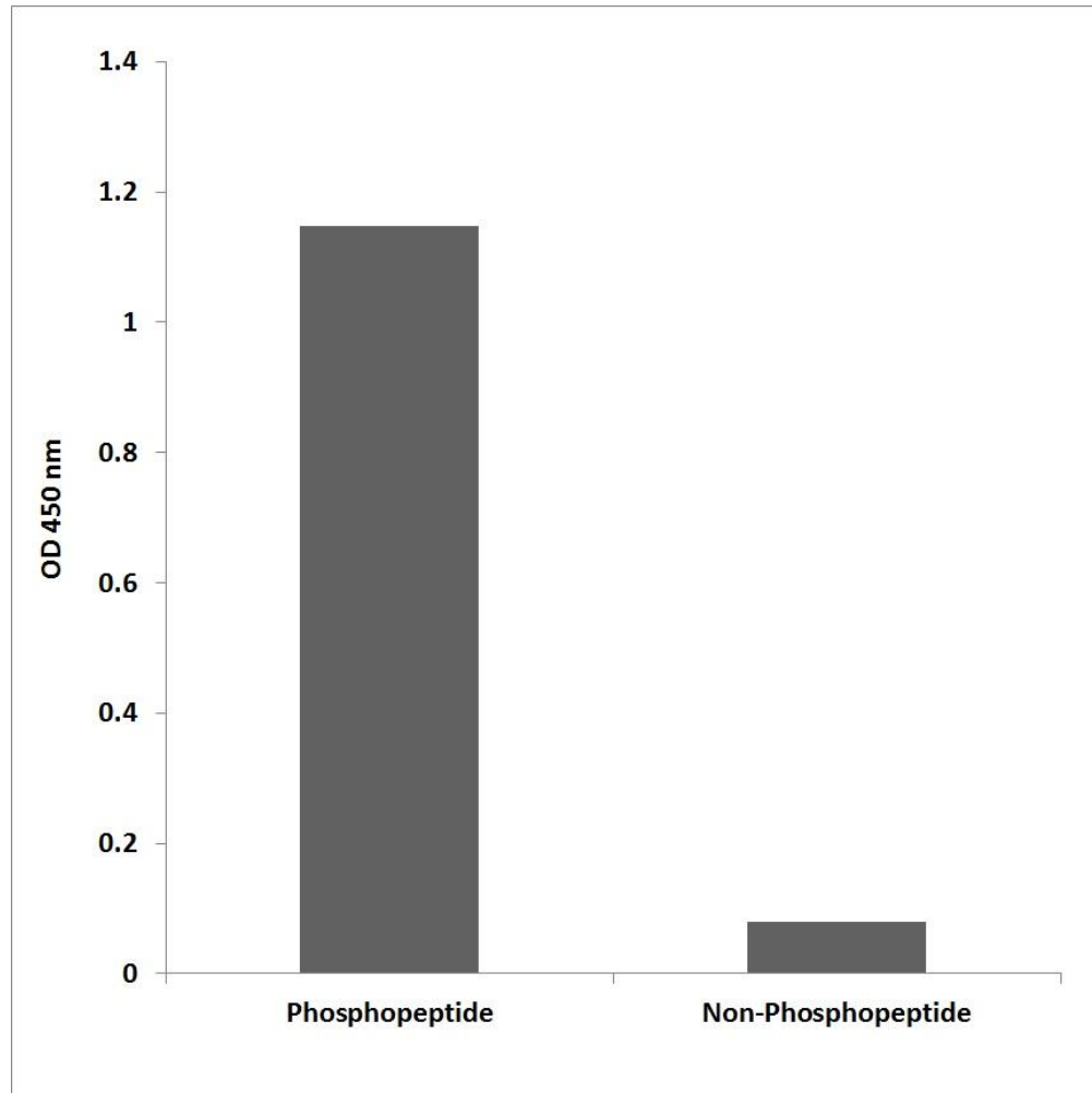
Figure 3. Enzyme-Linked Immunosorbent Assay (ELISA) for immunogen phosphor-peptide (left) and non-phospho peptide (right), using Anti-GRB10 (Phospho-Tyr67) Antibody.
