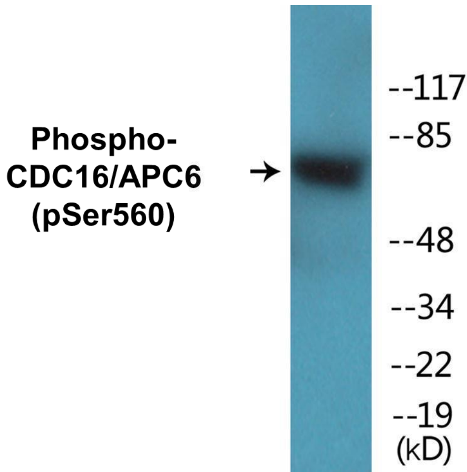
Figure 2. Western blot analysis of extracts from HuvEc cells, using the Anti-CDC16/APC6 (Phospho-Ser560) Antibody.
