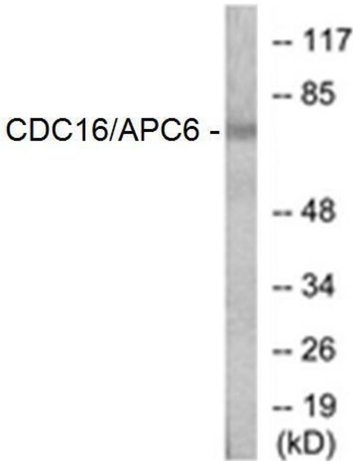
Figure 4. Western blot analysis of extracts from HuvEc cells, using the Anti-CDC16/APC6 Antibody.
