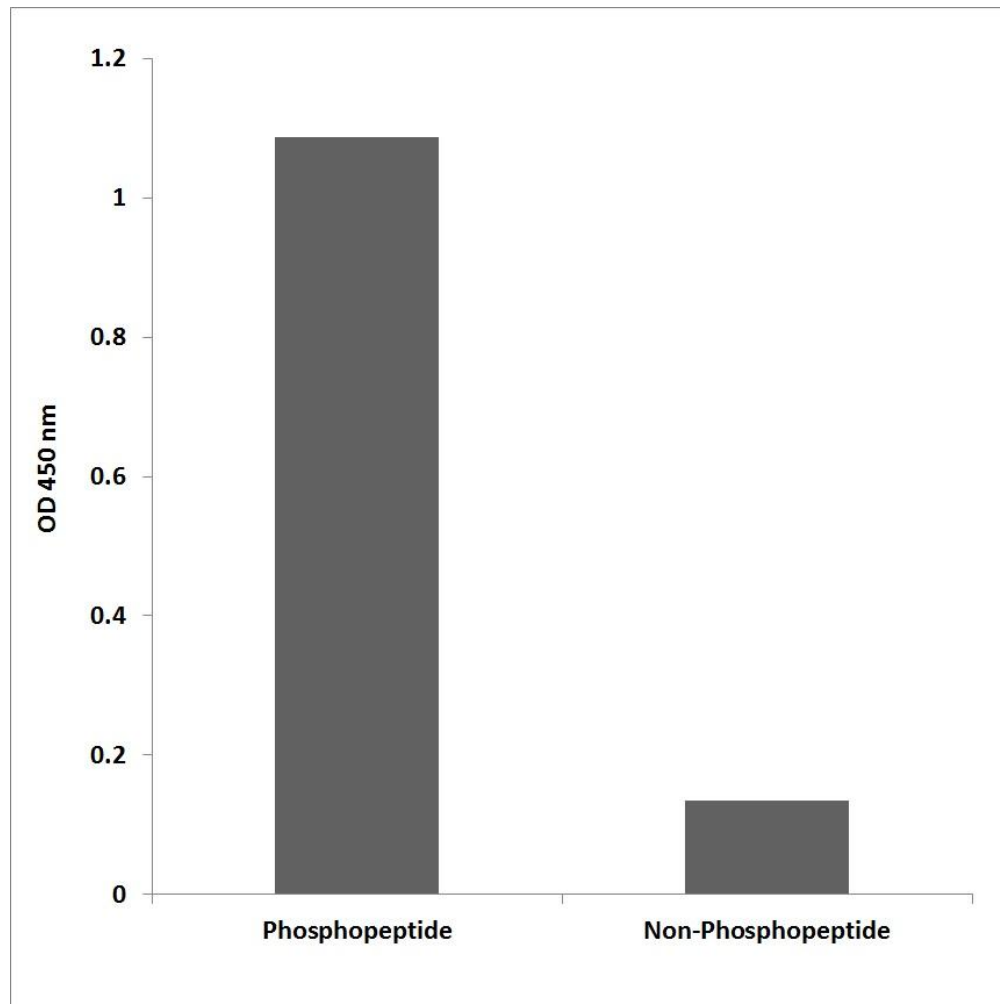
Figure 3. Enzyme-Linked Immunosorbent Assay (ELISA) for immunogen phosphor-peptide (left) and non-phospho peptide (right), using Anti-CDC16/APC6 (Phospho-Ser560) Antibody.
