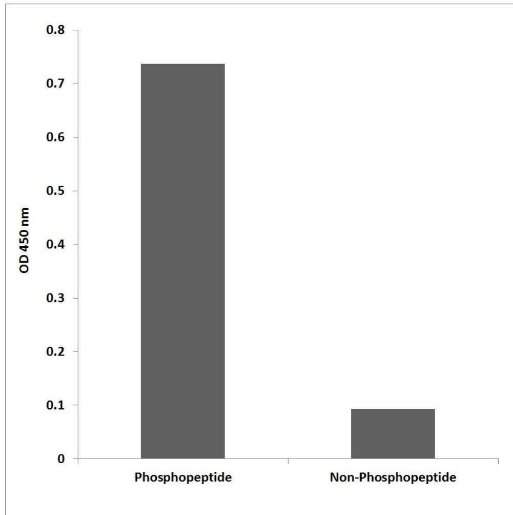
Figure 3. Enzyme-Linked Immunosorbent Assay (ELISA) for immunogen phosphor-peptide (left) and non-phospho peptide (right), using Anti-Smad1 (Phospho-Ser187) Antibody.
