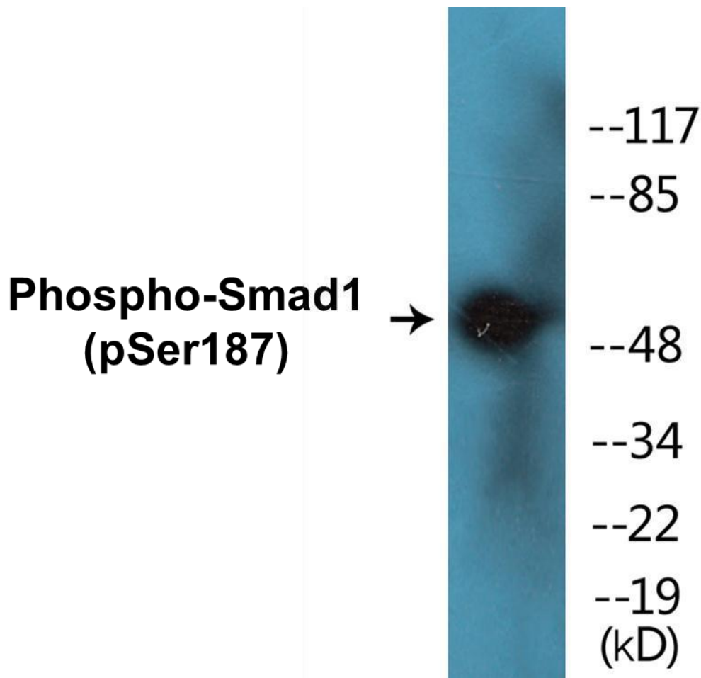
Figure 2. Western blot analysis of extracts from 293 cells and HepG2 cells, using the Anti-Smad1 (Phospho-Ser187) Antibody.
