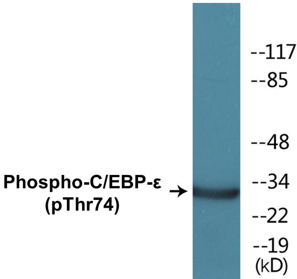
Figure 2. Western blot analysis of extracts from HuvEc cells treated with UV 15', using the Anti-C/EBP- \epsilon (Phospho-Thr74) Antibody.
