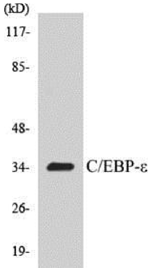
Figure 4. Western blot analysis of extracts from JurKat cells, treated with Insulin 0.01U/ml 15', using the Anti-C/EBP-ε Antibody.
