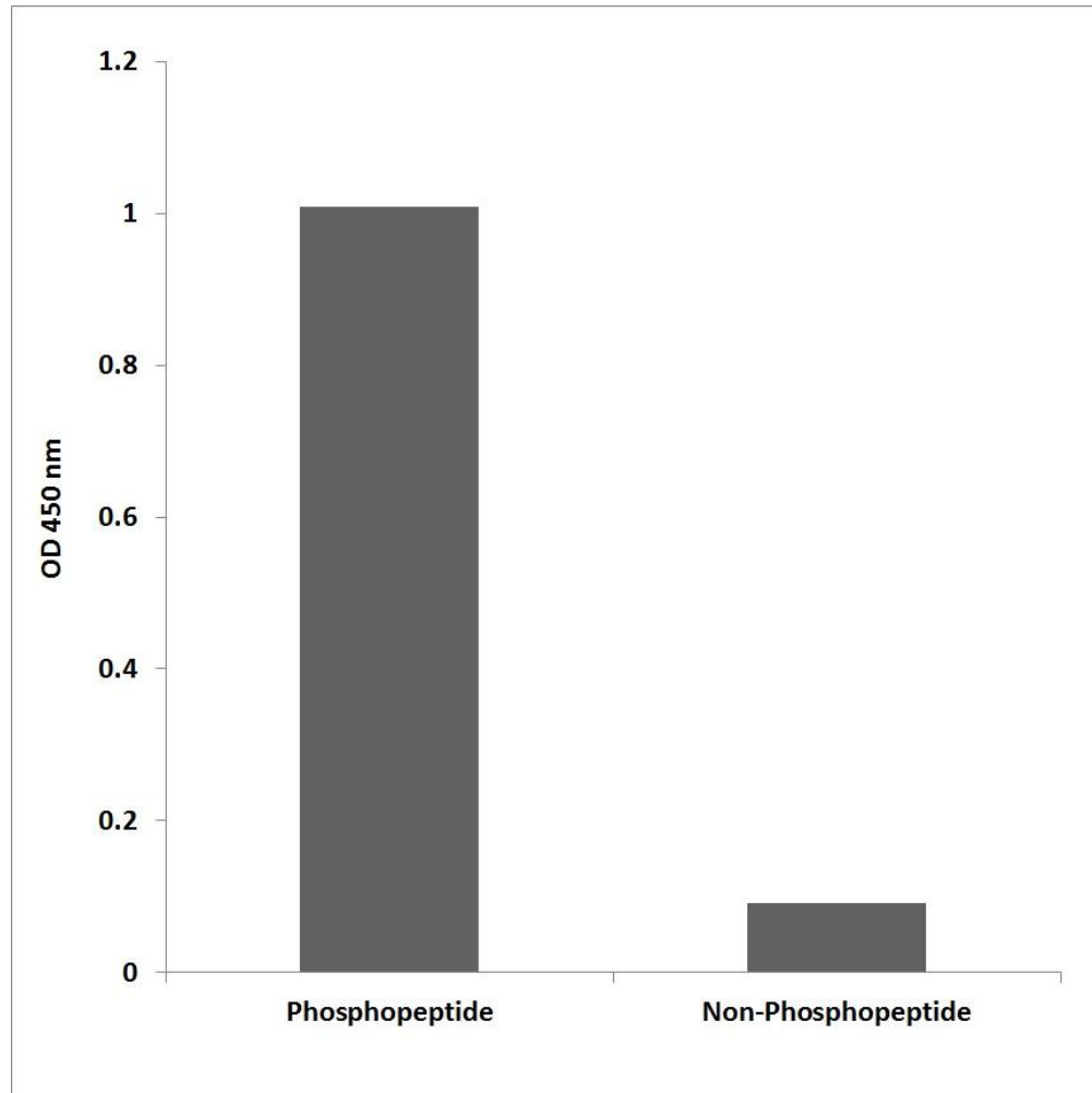
Figure 3. Enzyme-Linked Immunosorbent Assay (ELISA) for immunogen phosphor-peptide (left) and non-phospho peptide (right), using Anti-C/EBP- \epsilon (Phospho-Thr74) Antibody.
