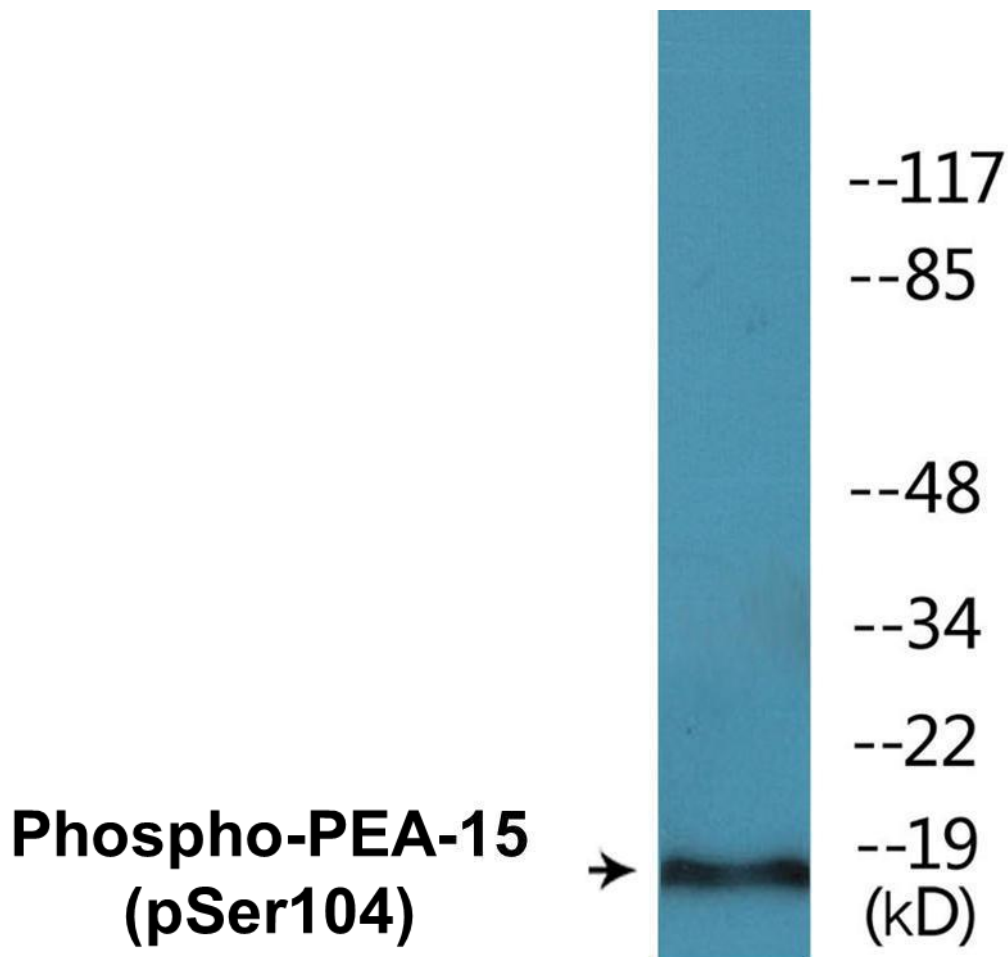
Figure 2. Western blot analysis of extracts from COS7 cells treated with TNF 20ng/ml 5', using the Anti-PEA-15 (Phospho-Ser104) Antibody
