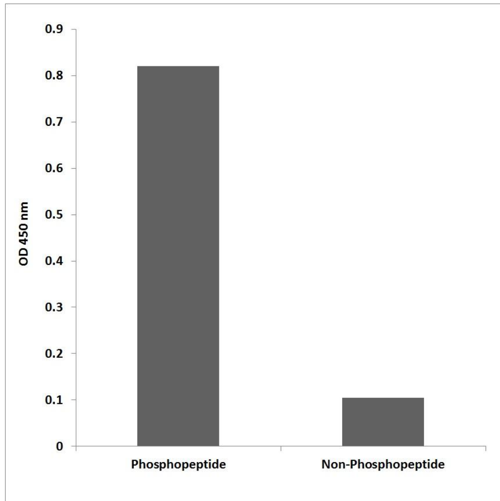
Figure 3. Enzyme-Linked Immunosorbent Assay (ELISA) for immunogen phosphor-peptide (left) and non-phospho peptide (right), using Anti-PEA-15 (Phospho-Ser104) Antibody.
