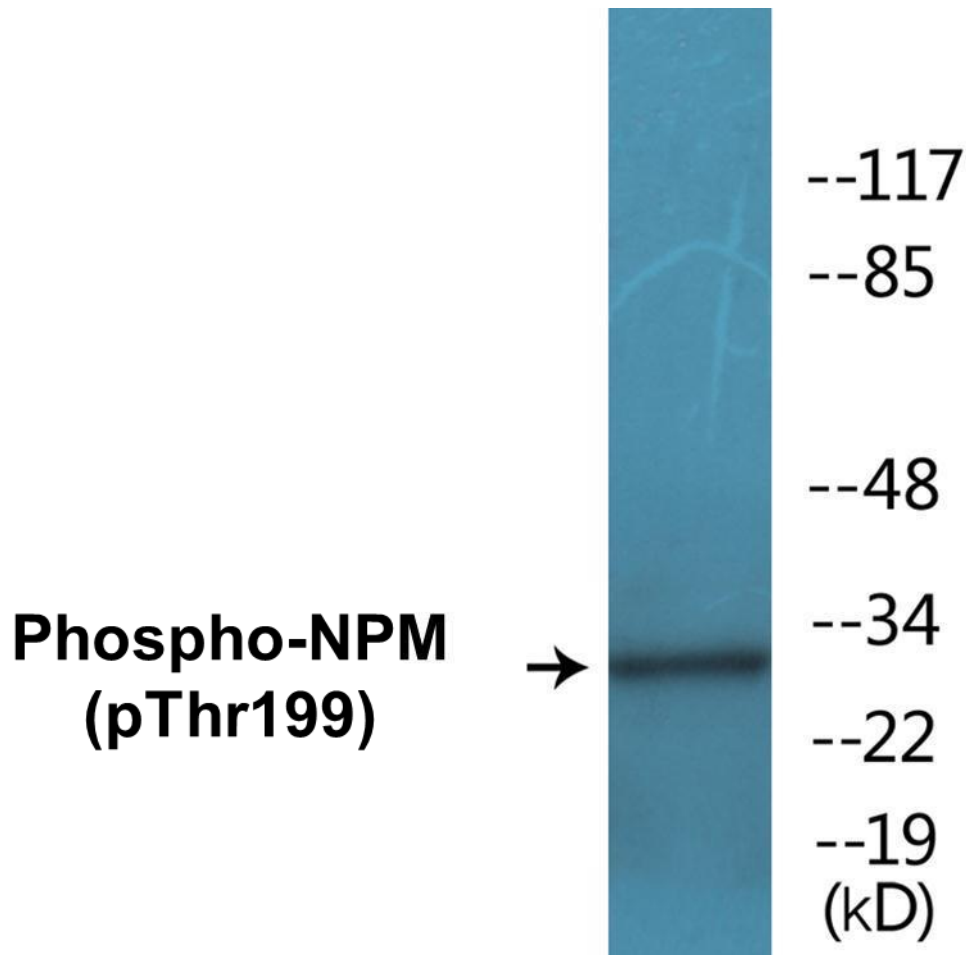
Figure 2. Western blot analysis of extracts from HepG2 cells, using the Anti-NPM (Phospho-Thr199) Antibody.
