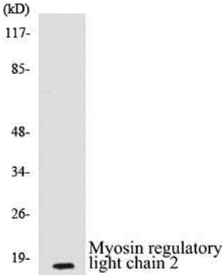
Figure 4. Western blot analysis of extracts from COLO205 cells, using the Anti-Myosin regulatory light chain 2 Antibody.
