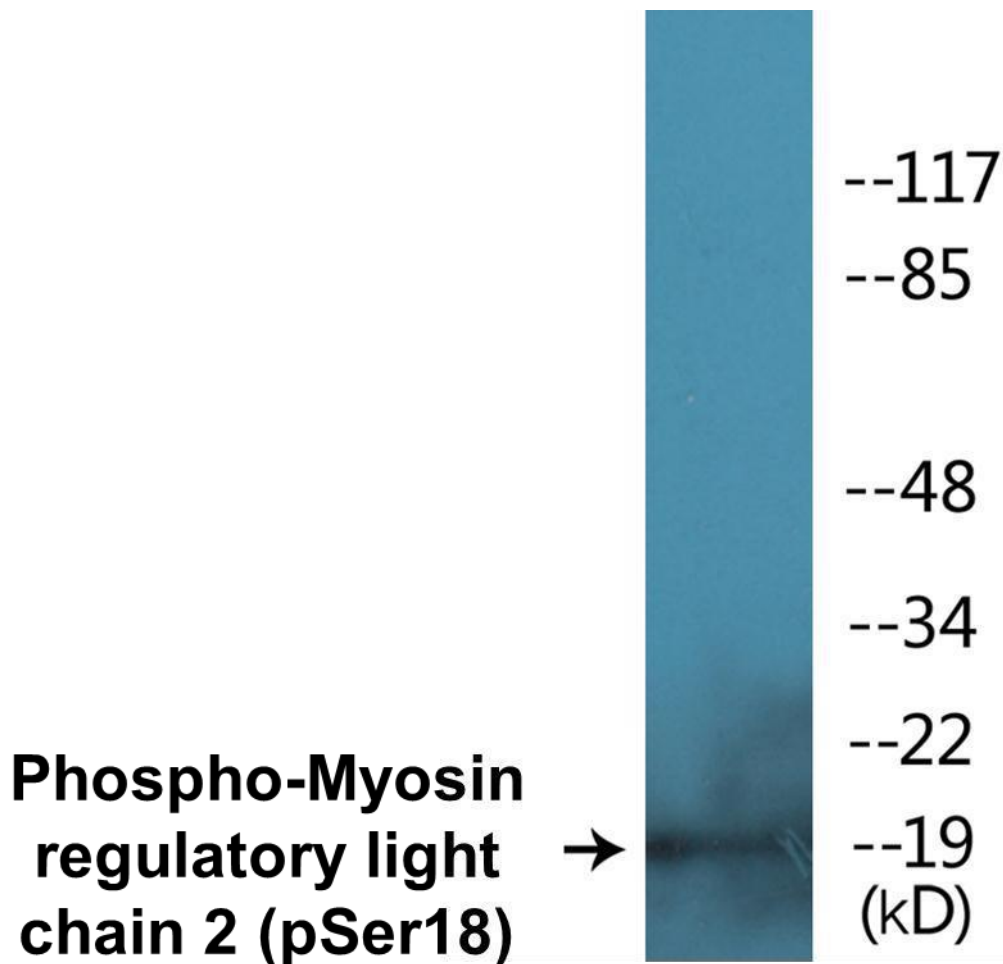
Figure 2. Western blot analysis of extracts from LOVO cells treated with H 2 O 2 -Ser18) Antibody.
