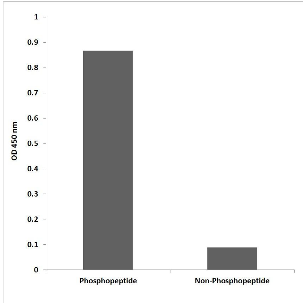
Figure 3. Enzyme-Linked Immunosorbent Assay (ELISA) for immunogen phosphor-peptide (left) and non-phospho peptide (right), using Anti-Mst1/2 (Phospho-Thr183) Antibody.
