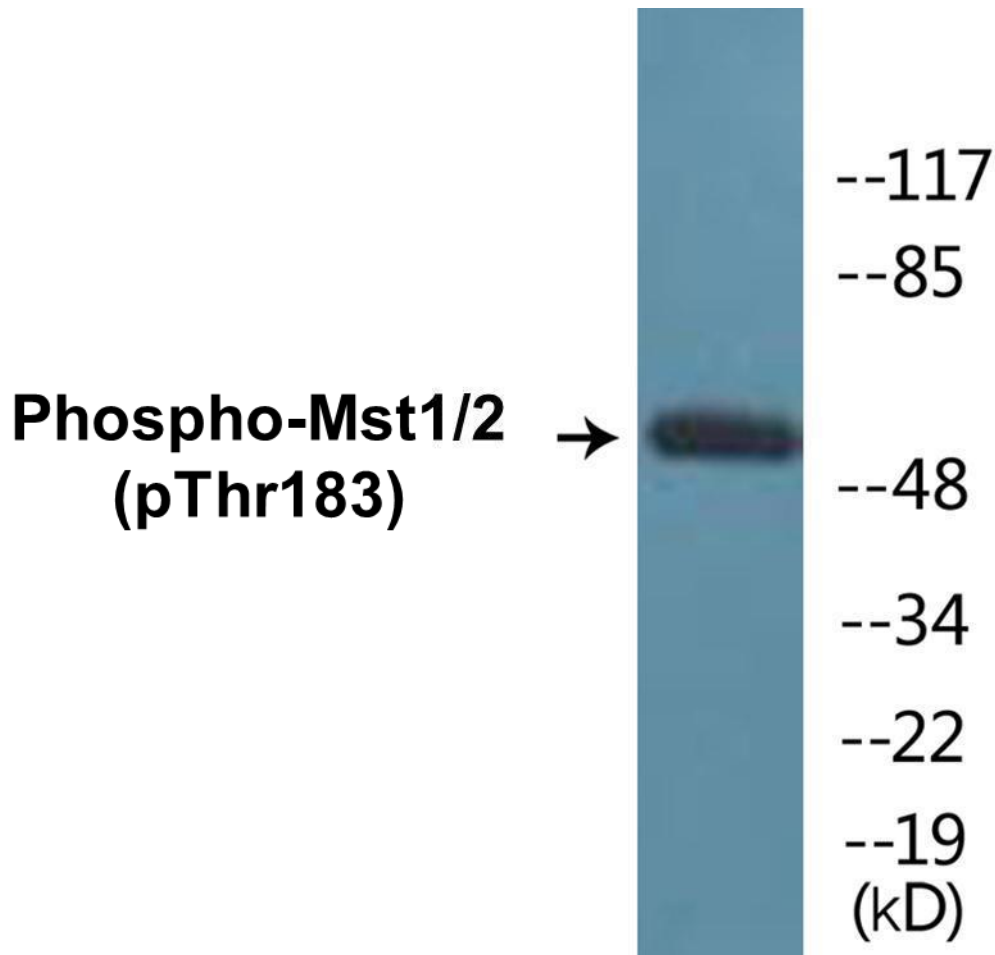
Figure 2. Western blot analysis of extracts from 293 cells treated with H 2 O 2 100uM 15', using the Anti-Mst1/2 (Phospho-Thr183) Antibody.
