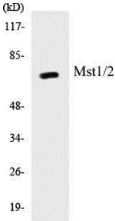
Figure 4. Western blot analysis of extracts from HeLa cells, treated with UV 15', using the Anti-Mst1/2 Antibody.
