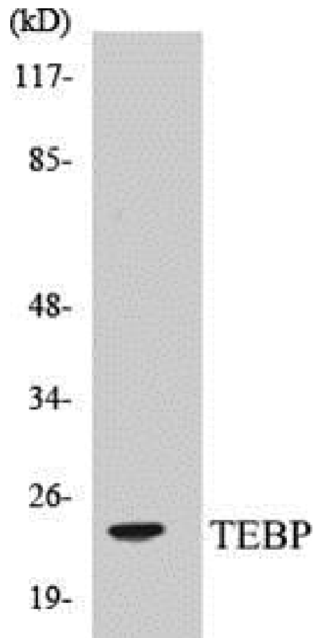
Figure 4. Western blot analysis of extracts from NIH-3T3 cells, treated with EGF 200ng/ml 30', using the Anti-TEBP Antibody.
