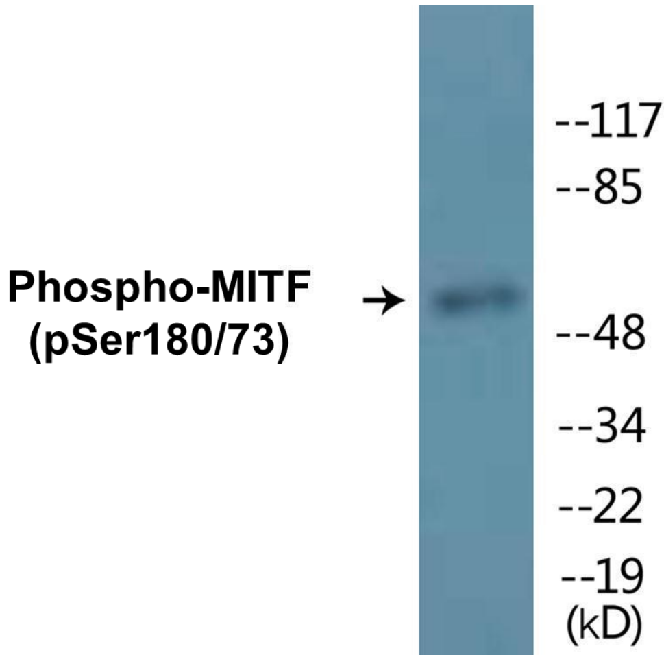
Figure 2. Western blot analysis of extracts from COS7 cells, using the Anti-MITF (Phospho-Ser180/73) Antibody.
