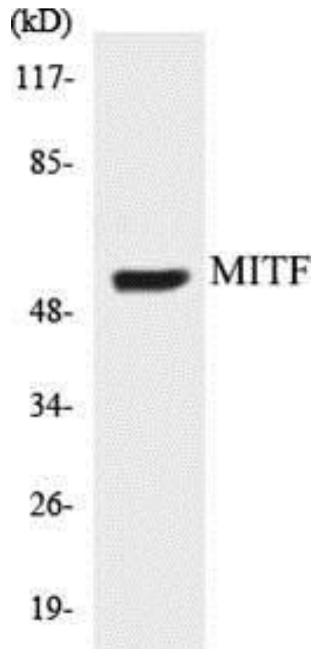
Figure 4. Western blot analysis of extracts from HepG2 cells, using the Anti-MITF Antibody.
