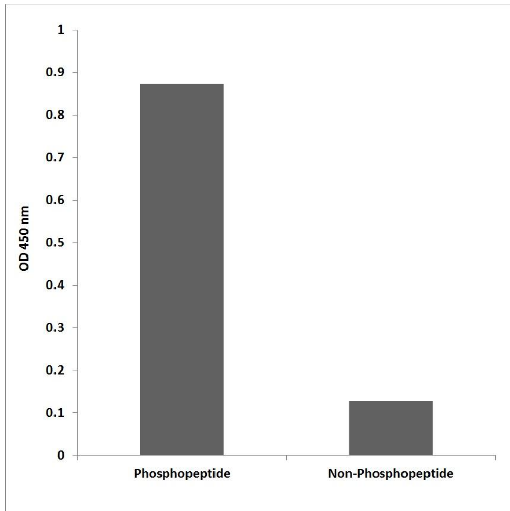
Figure 3. Enzyme-Linked Immunosorbent Assay (ELISA) for immunogen phosphor-peptide (left) and non-phospho peptide (right), using Anti-MITF (Phospho-Ser180/73) Antibody.
