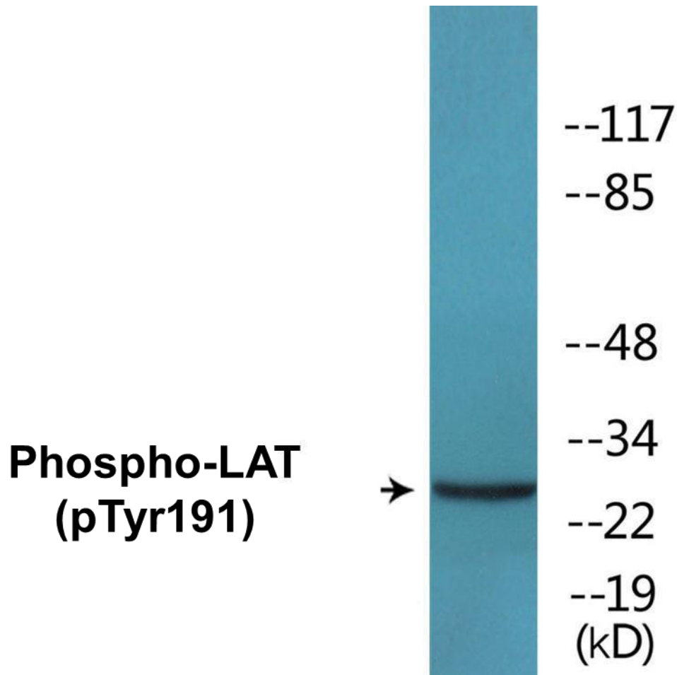
Figure 2. Western blot analysis of extracts from NIH-3T3 cells, using the Anti-LAT (Phospho-Tyr191) Antibody.
