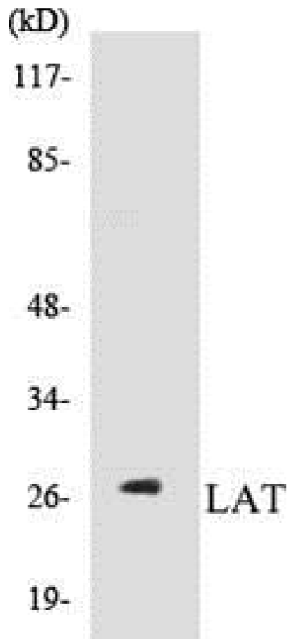
Figure 4. Western blot analysis of extracts from NIH-3T3 cells, using the Anti-LAT Antibody.
