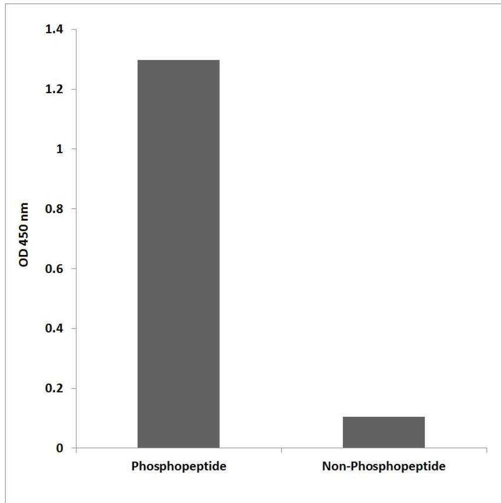
Figure 3. Enzyme-Linked Immunosorbent Assay (ELISA) for immunogen phosphor-peptide (left) and non-phospho peptide (right), using Anti-LAT (Phospho-Tyr191) Antibody.
