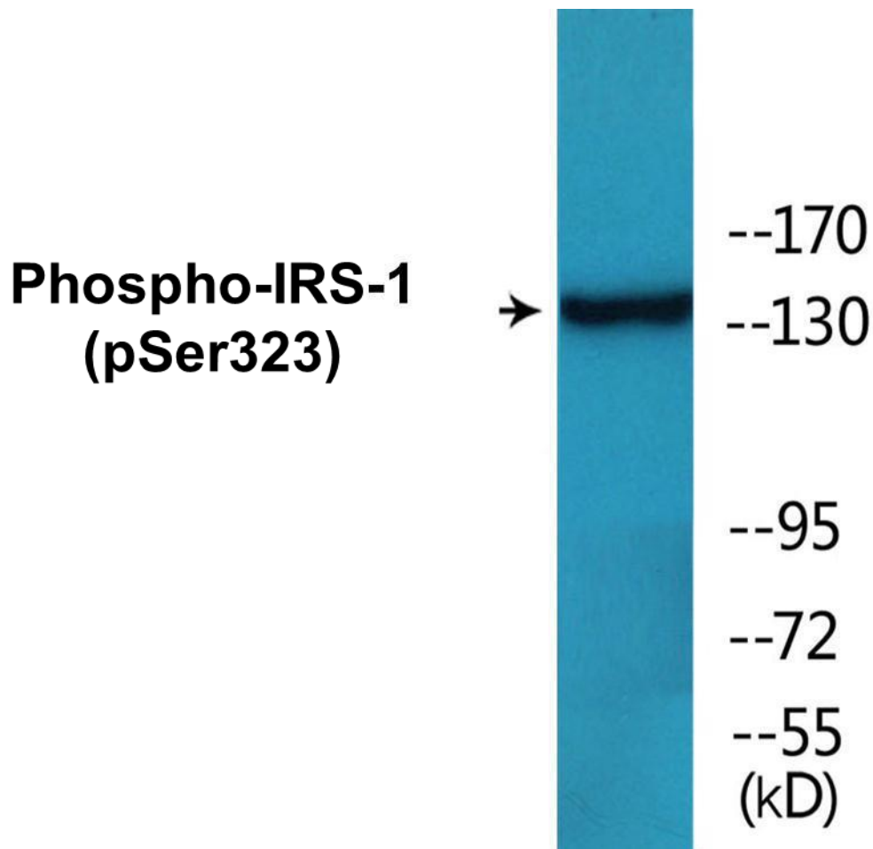
Figure 2. Western blot analysis of extracts from COS7 cells treated with Serum 20% 15', using the Anti-IRS-1 (Phospho-Ser323) Antibody.
