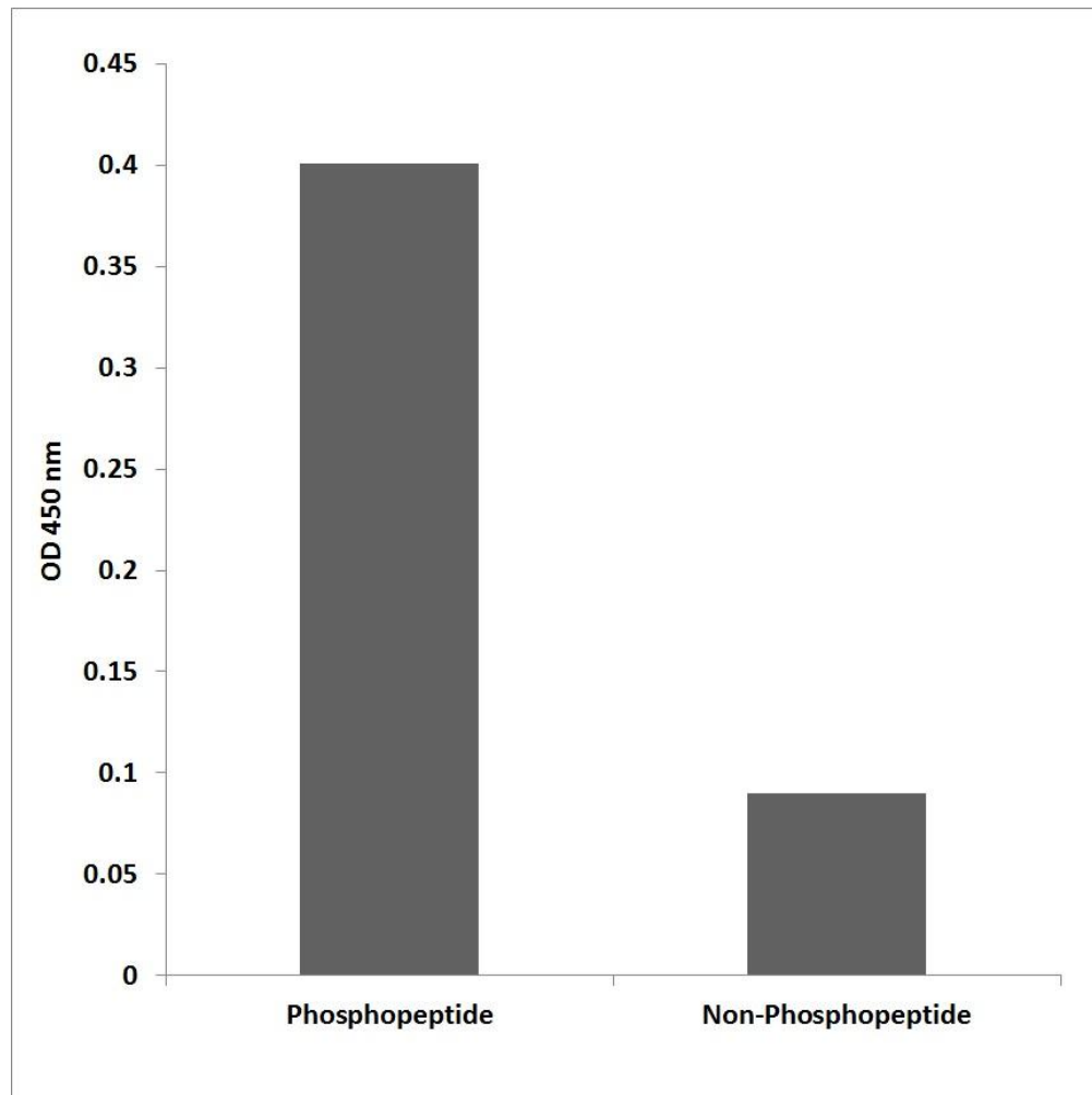
Figure 3. Enzyme-Linked Immunosorbent Assay (ELISA) for immunogen phosphor-peptide (left) and non-phospho peptide (right), using Anti-IRS-1 (Phospho-Ser323) Antibody.
