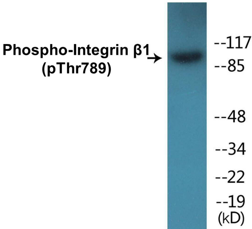
Figure 2. Western blot analysis of extracts from HepG2 cells treated with \text{Ca}^{2+} 40 \mu\text{M} 30', using the Anti-Integrin \beta 1 (Phospho-Thr789) Antibody.
