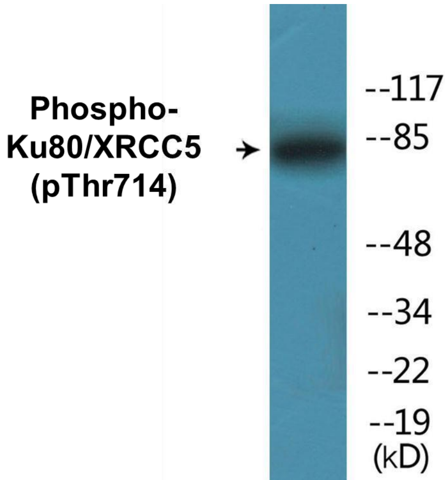
Figure 2. Western blot analysis of extracts from COS7 cells, using the Anti-Ku80/XRCC5 (Phospho-Thr714) Antibody.
