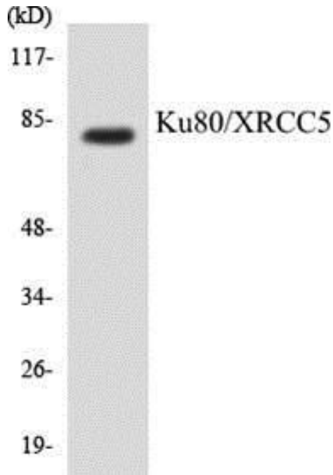
Figure 4. Western blot analysis of extracts from COS7 cells, using the Anti-Ku80/XRCC5 Antibody.
