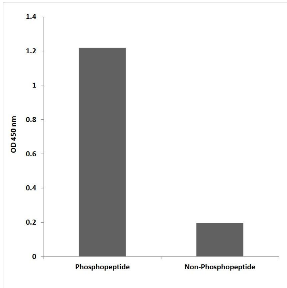
Figure 3. Enzyme-Linked Immunosorbent Assay (ELISA) for immunogen phosphor-peptide (left) and non-phospho peptide (right), using Anti-Ku80/XRCC5 (Phospho-Thr714) Antibody.
