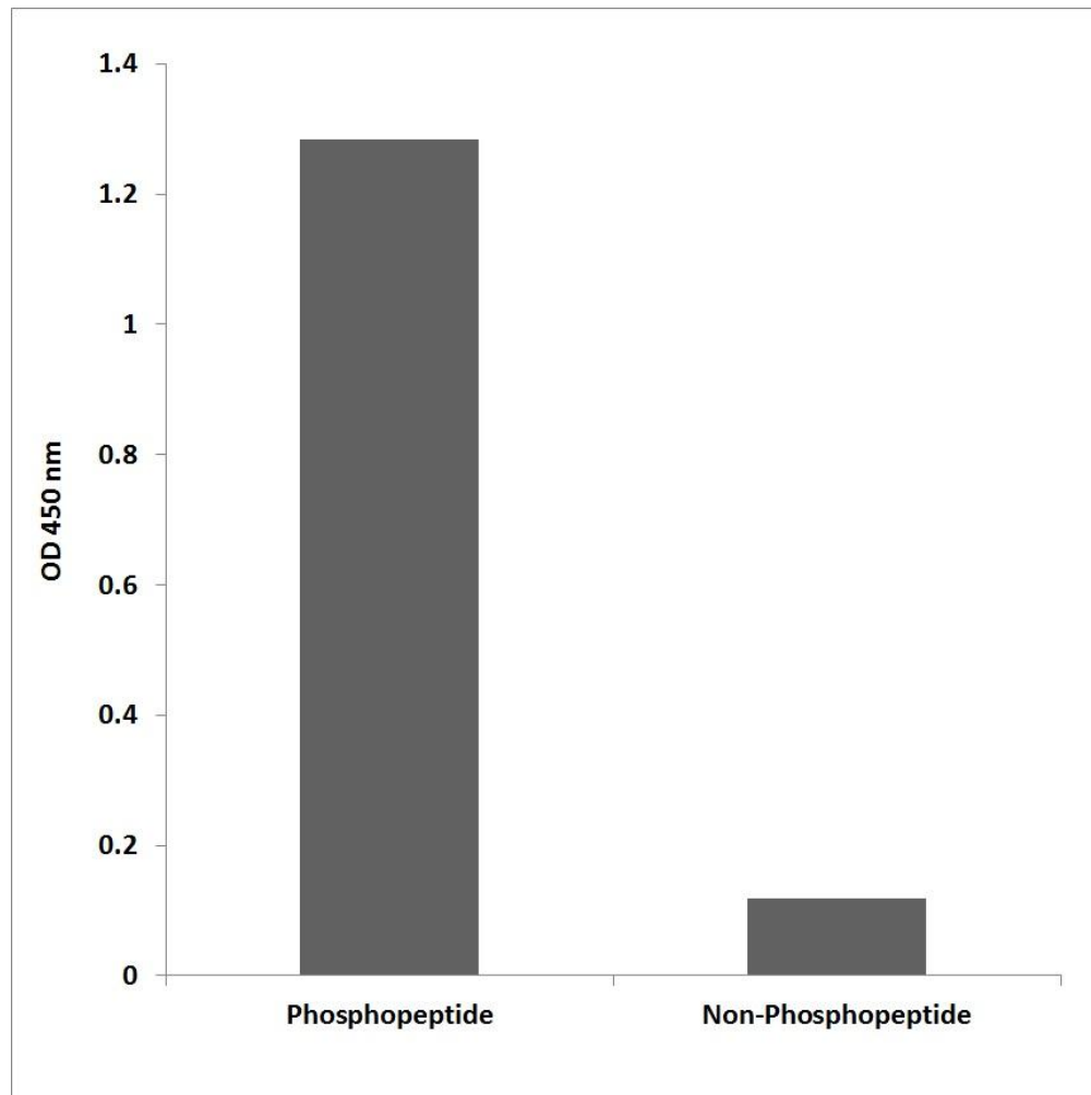
Figure 3. Enzyme-Linked Immunosorbent Assay (ELISA) for immunogen phosphor-peptide (left) and non-phospho peptide (right), using Anti-HSL (Phospho-Ser552) Antibody.
