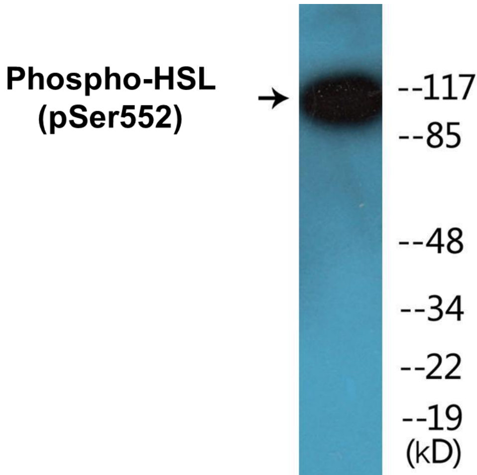
Figure 2. Western blot analysis of extracts from K562 cells, using the Anti-HSL (Phospho-Ser552) Antibody.
