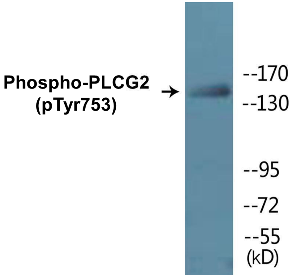
Figure 2. Western blot analysis of extracts from HepG2 cells treated with Na 3 VO 4 0.3mM 40', using the Anti-PLCG2 (Phospho-Tyr753) Antibody.
