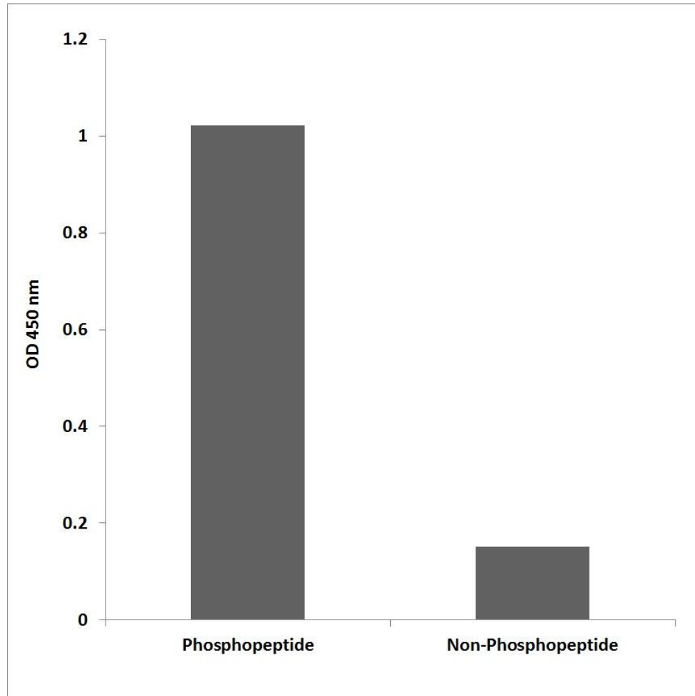
Figure 3. Enzyme-Linked Immunosorbent Assay (ELISA) for immunogen phosphor-peptide (left) and non-phospho peptide (right), using Anti-PLCG2 (Phospho-Tyr753) Antibody.
