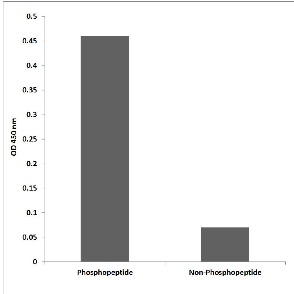
Figure 3. Enzyme-Linked Immunosorbent Assay (ELISA) for immunogen phosphor-peptide (left) and non-phospho peptide (right), using Anti-MAP3K8 (Phospho-Thr290) Antibody.
