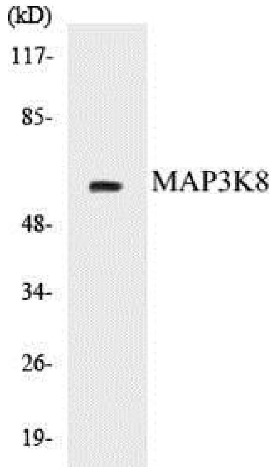
Figure 4. Western blot analysis of extracts from COLO205 cells, treated with Insulin 0.01U/ml 15', using the Anti-MAP3K8 Antibody.
