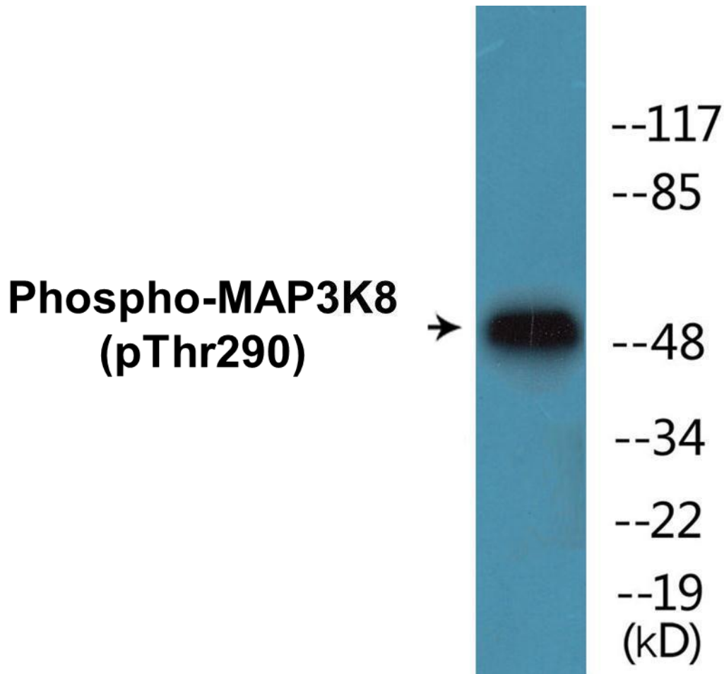
Figure 2. Western blot analysis of extracts from 293 cells treated with UV 15', using the Anti-MAP3K8 (Phospho-Thr290) Antibody.
